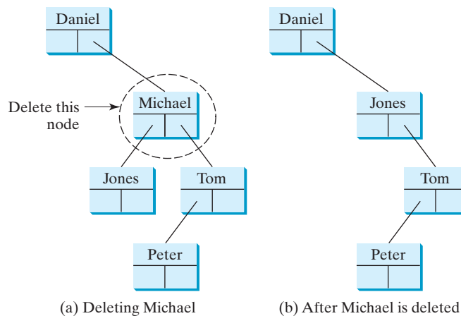
FIGURE 25.16 Deleting Michael falls into Case 2.
