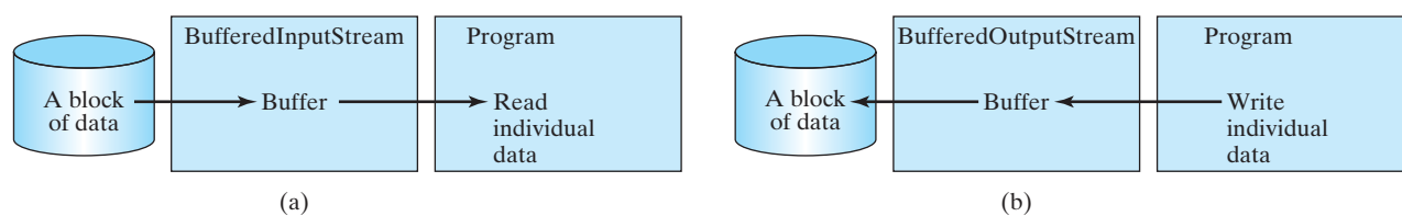
FIGURE 17.12 Buffer I/O places data in a buffer for fast processing.
