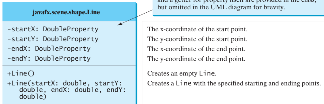
FIGURE 14.28 The Line class defines a line.
