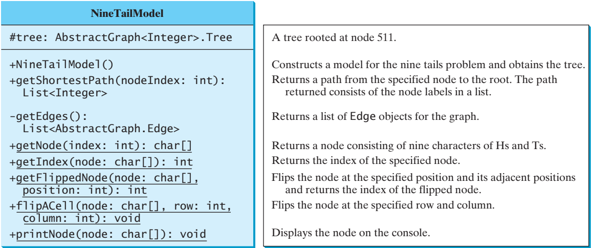
FIGURE 28.20 The NineTailModel class models the nine tails problem using a graph.
