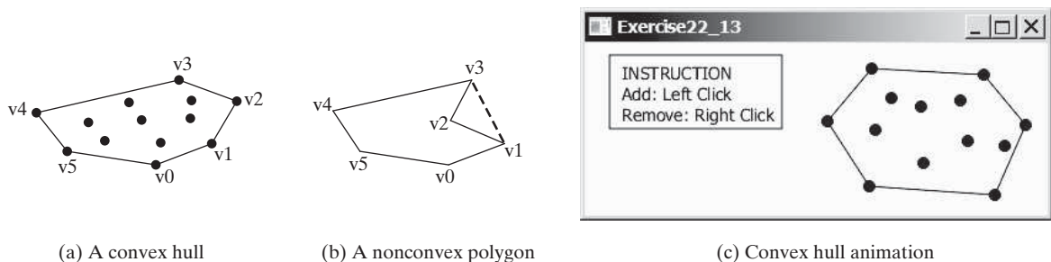
FIGURE 22.8 A convex hull is the smallest convex polygon that contains a set of points.
