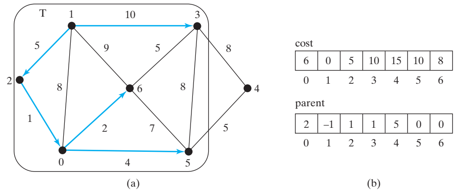
FIGURE 29.17 Now vertices {1, 2, 0, 6, 3, 5} are in set T .
